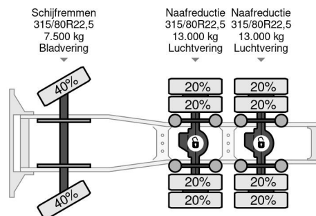
MAN 26.403 DFS 6x4 TRACTOR UNIT (EURO 2 / MANUAL ...
