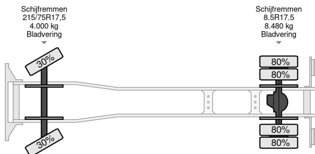
Renault Midlum 180 4x2 FULL STEEL SUSPENSION CHASS...
