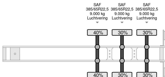
Schmitz Cargobull SCS 24/L 3-AXLE FLATBED TRAILER (D...
