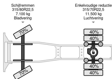
Renault Magnum AE 480 E-TECH (MACK ENGINE / Z... 4x2
