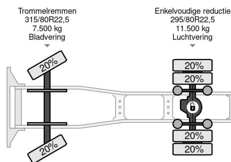
DAF 95.480 XF SPACECAB (EURO 3 / ZF16 MANUAL ... 4x2
