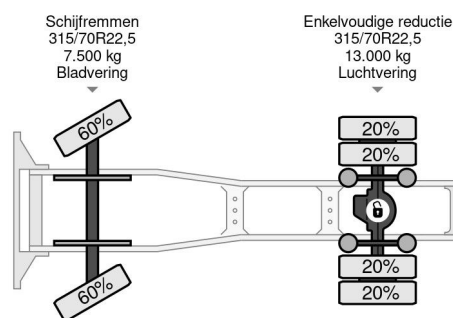
DAF XF 105.460 SPACECAB (ZF16 MANUAL GEARBOX / MX-BRAKE / 870+430 LITER TANK / AIRCONDITIONING / FRIDGE) 4x2
