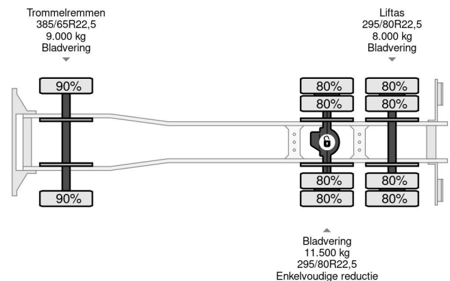
Scania P114-340 6x2 WITH MULTILIFT CONTAINERSYSTEM...
